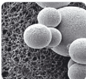
Chromatography gel beads (right) are shown on top of a membrane adsorber in this SEM picture. The membrane adsorber pores are over 50 × larger than bead pores.
